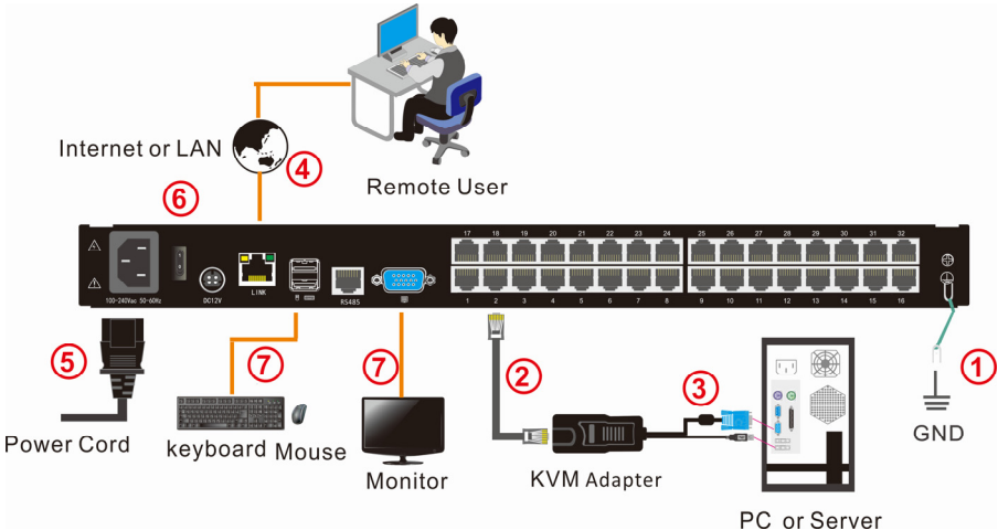
Figure 2.2 Installation diagram
