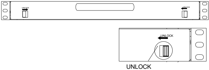
Figure 2.3 Unlocking
