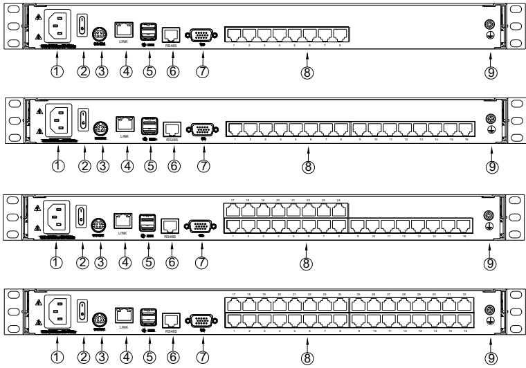
Figure 1.3 Rear view
