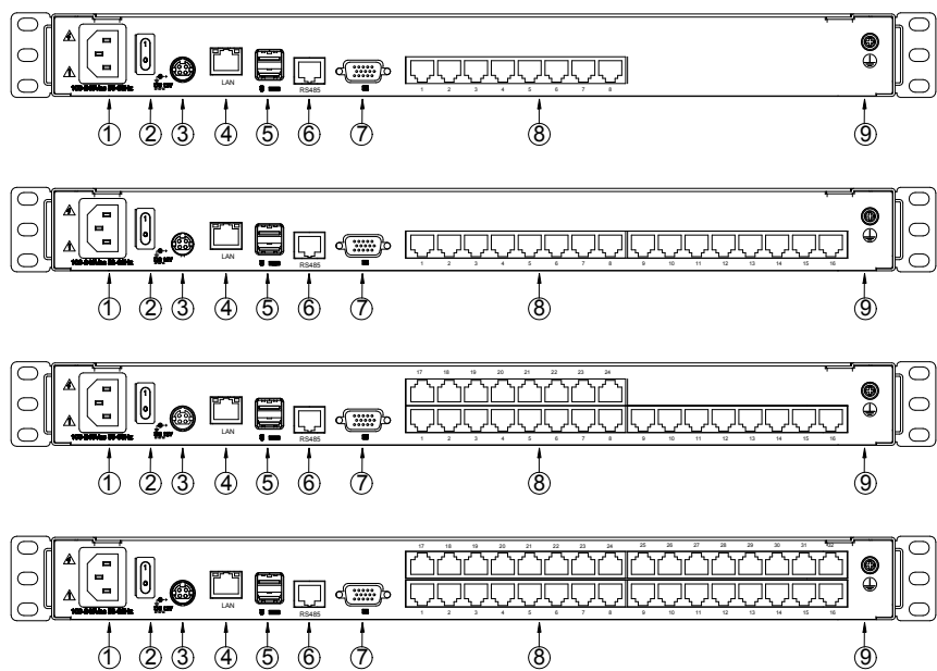
Figure 1.2 Rear view
