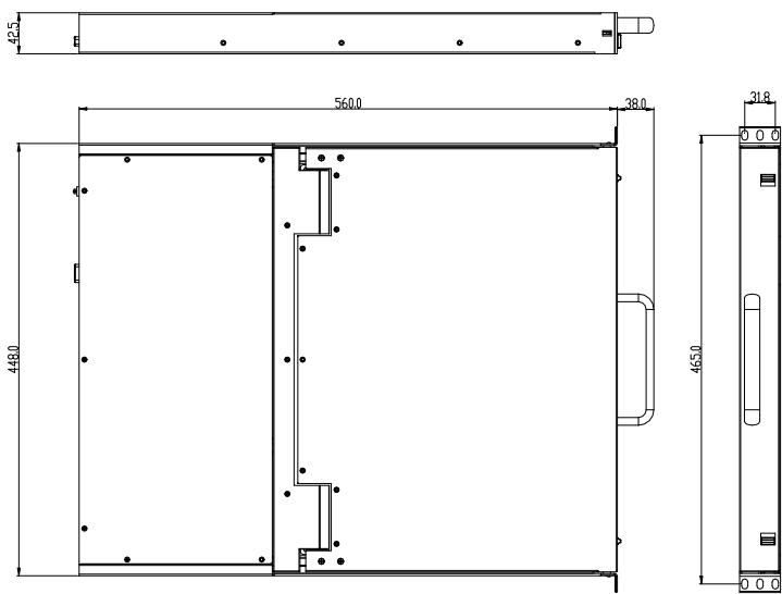
Figure 1.2 size dimensions
