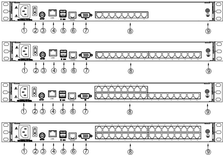
Figure 1.3 Rear view
