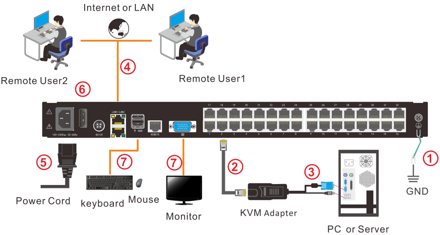
Figure 2.2 Installation diagram
