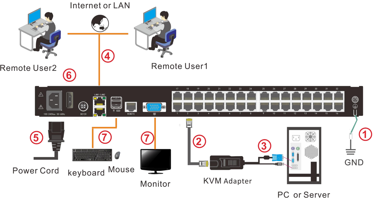
Figure 2.2 Installation Diagram
