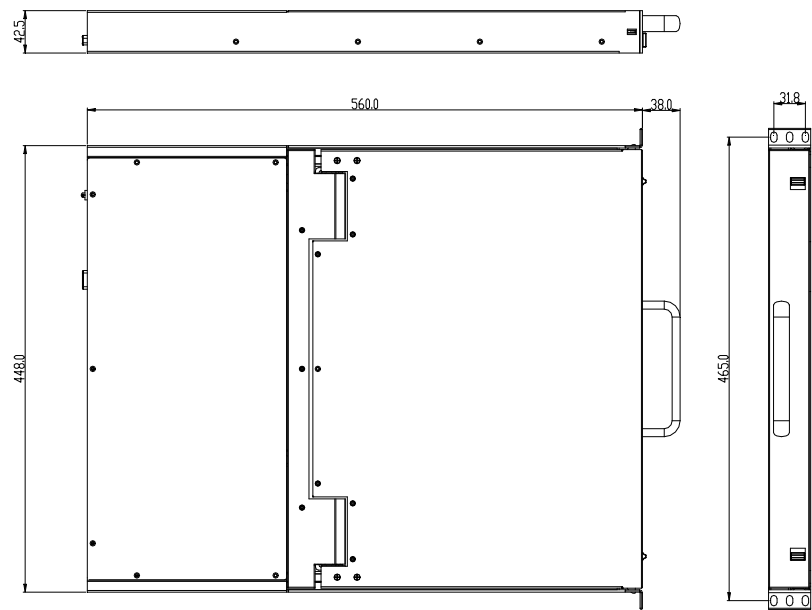
Figure 1.2 Size Dimension
