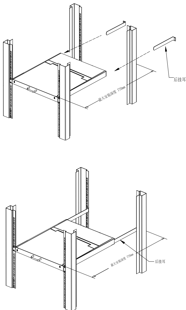
Figure 2.1 Rack Installation Diagram
