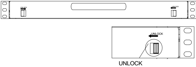
Figure 2.3 Unlocking
