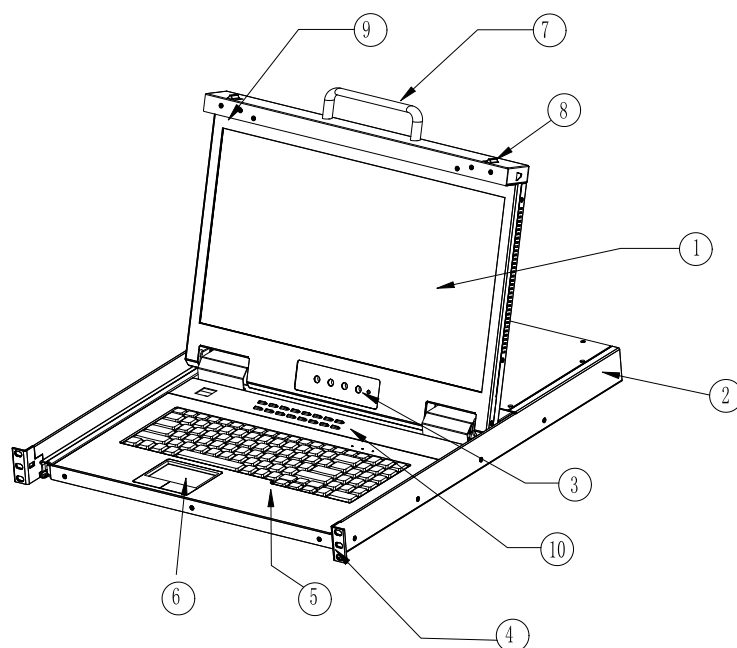
Figure 1.1 Front View
