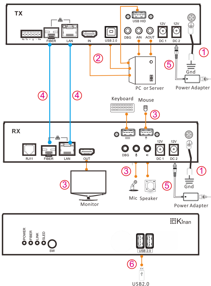
Connection Diagram of KFH186K
