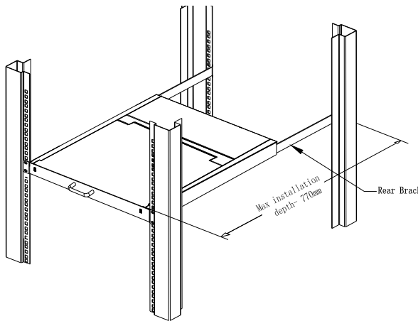
2-1.2 rack mounting (2)
