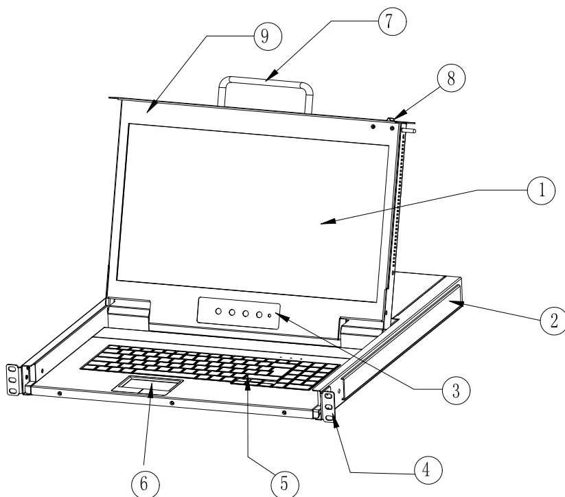
Figure 1-2 front view
