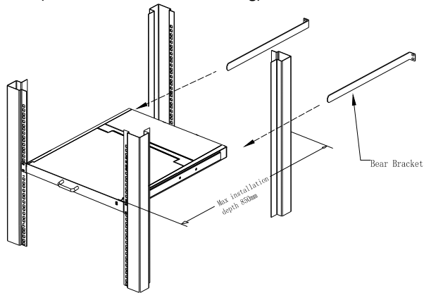
2-1.1 rack mounting (1)
