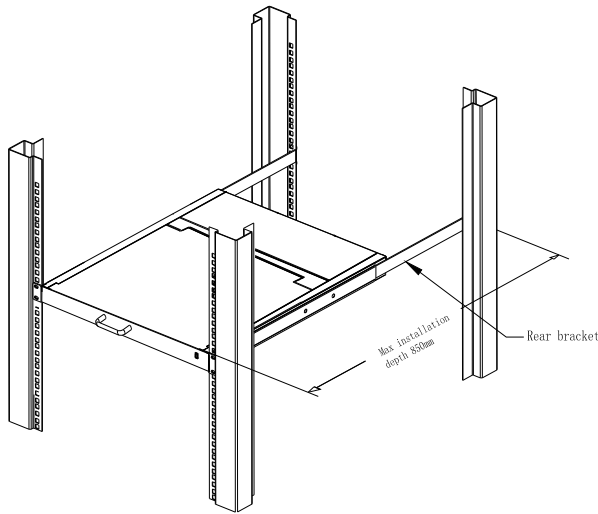
2-1.2 rack mounting (2)
