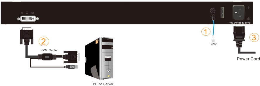
1-4 cable connection
