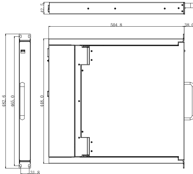
Figure 1-1 Appearance
