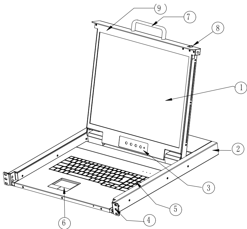
Figure 1-2 front view
