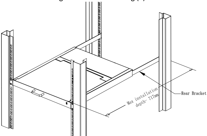
Figure 2-2 rack mounting (2)
