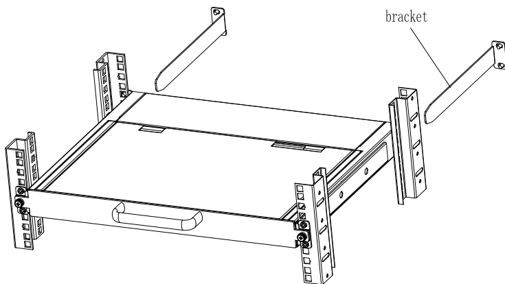
2-1.1 rack mounting (1)
