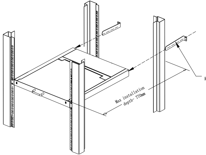
2-1.1 rack mounting (1)
