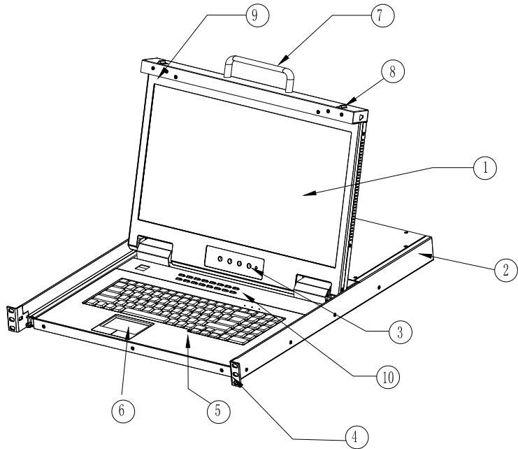
1-1.1 front view
