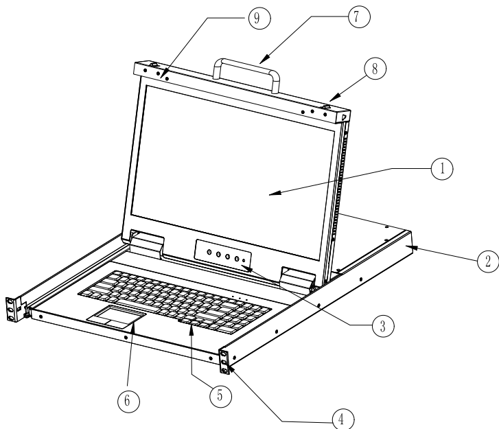
1-2 front view
