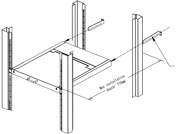
2-1 rack mounting
