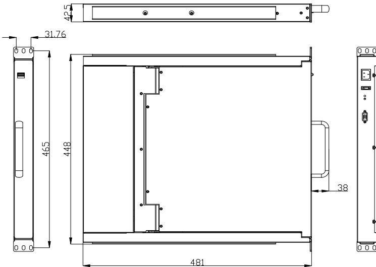
1-1 appearance
