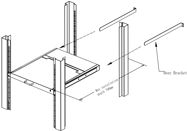
2-1 rack mounting (1)
