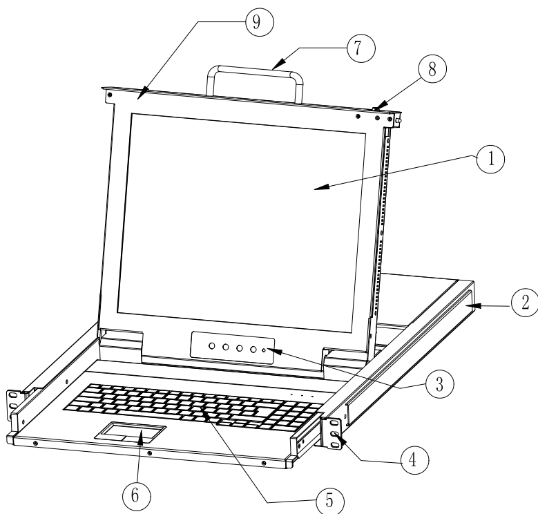
1-2 front view
