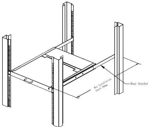
2-2 rack mounting (2)
