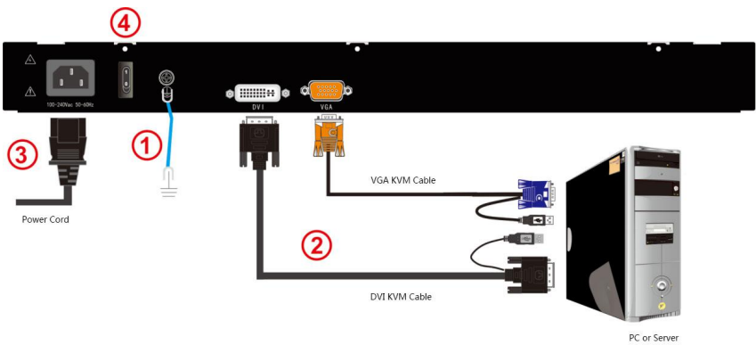
Figure 3-2 Connection Diagram
