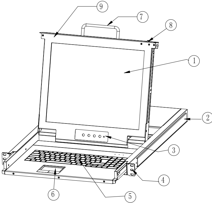
Figure 1-2 Front View
