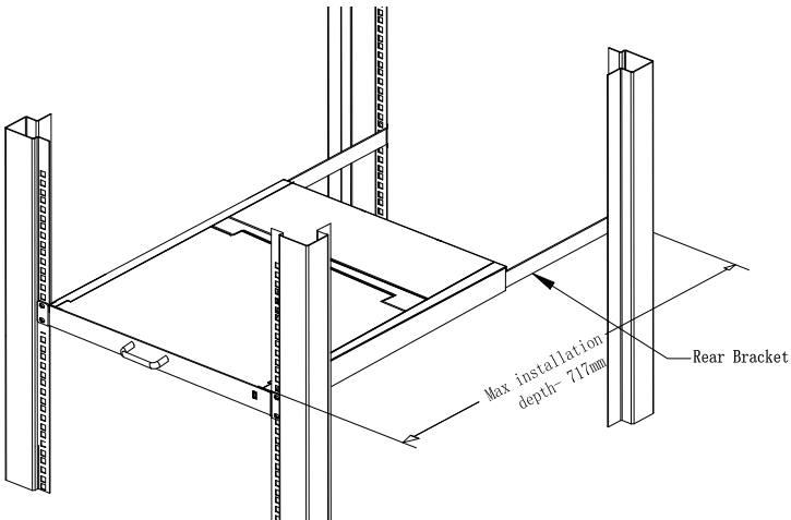
2-2 rack mounting (2)
