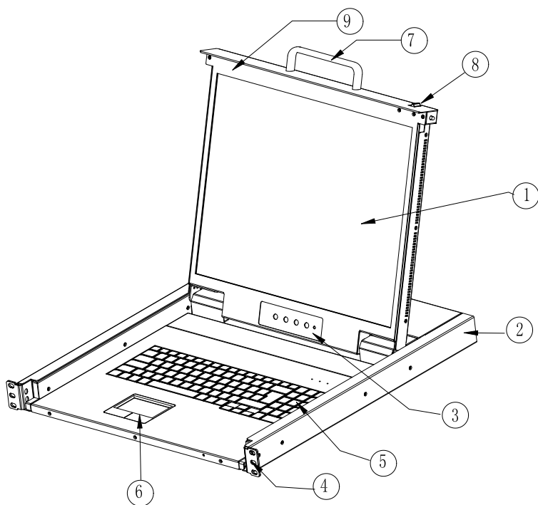
Figure 1-2 Front View
