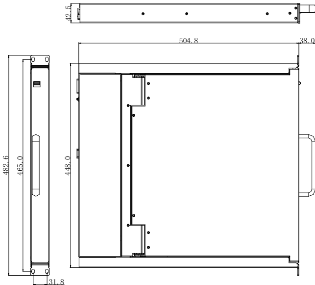
Figure 1-1 appearance
