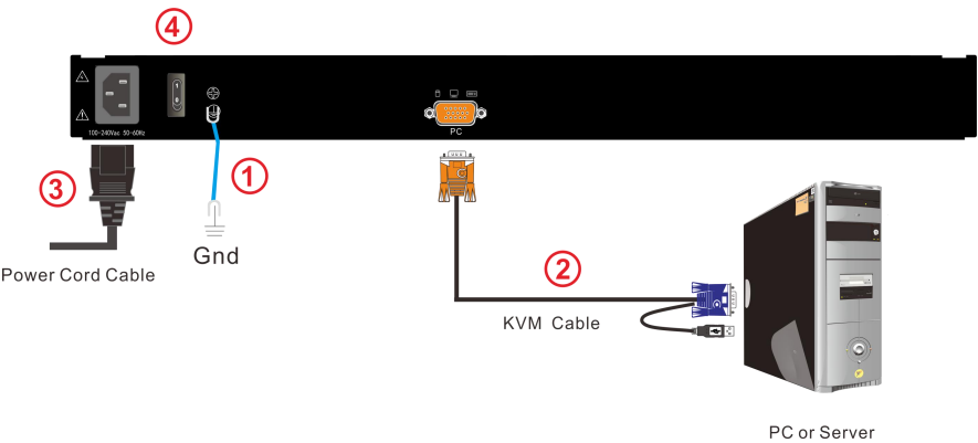
1-4 cable connection
