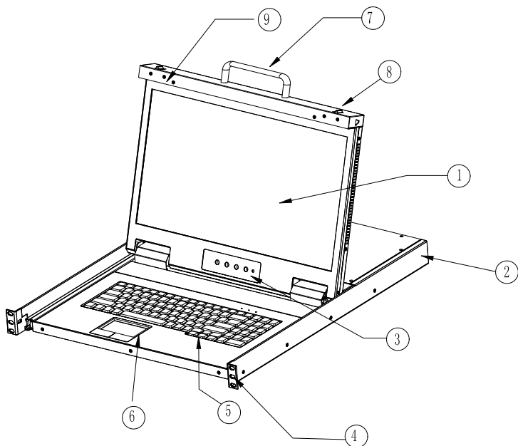
1-2 front view
