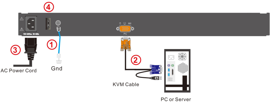
1-4 cable connection
