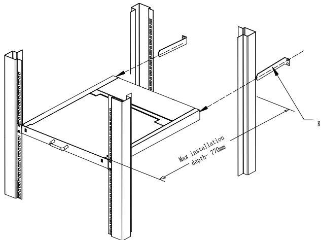
2-1 rack mounting
