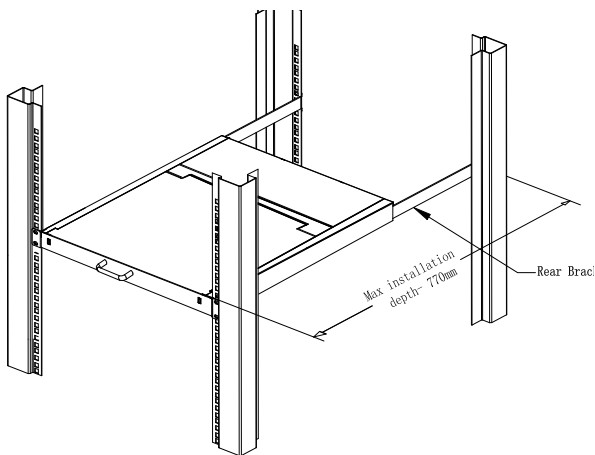
2-2 rack mounting
