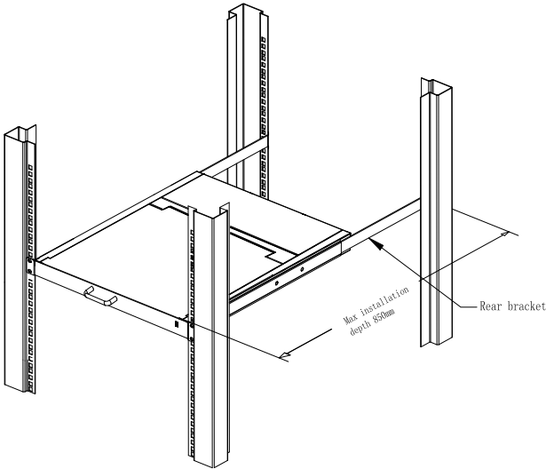
2-1.2 rack mounting (2)
