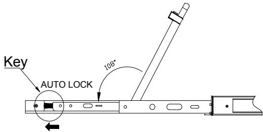
2-1.6 open angle of the console
