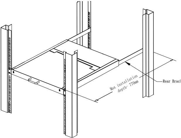
2-1.2 rack mounting (2)
