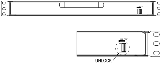
Figure 2-3.1 unlocking
