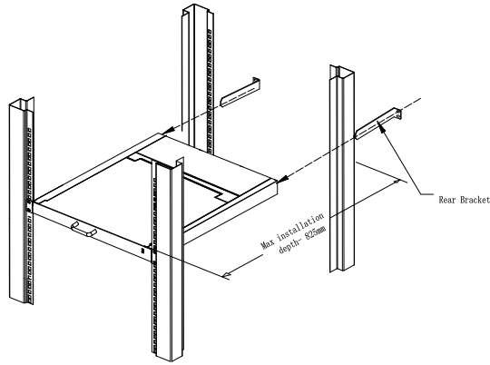
Figure 2-1.1 rack mounting (1)
