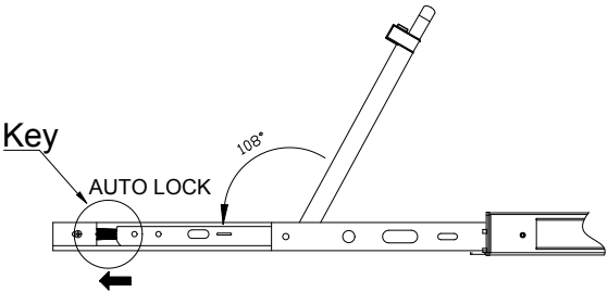
Figure 2-3.4 open angle of the console
