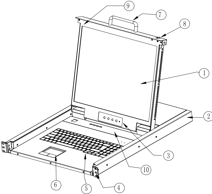
Figure 1-1.1 front view
