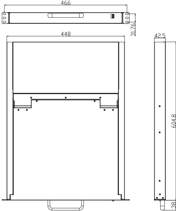
Figure 1-1.2 Appearance
