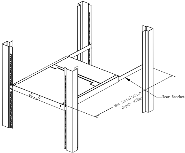
Figure 2-1.2 rack mounting (2)
