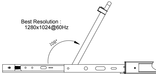
Figure 2-3.2 rotate angle of the console
