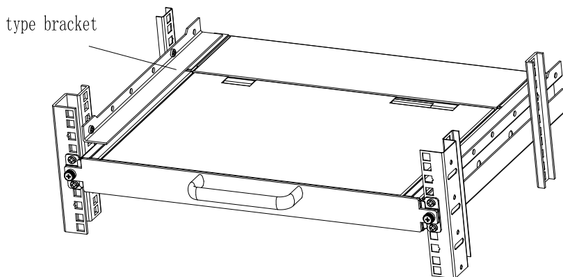
2-1.4 rack mounting (4)
