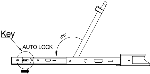
Diagram 2-1.6 unlocking the console
