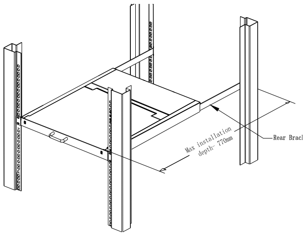
2-1.2 rack mounting (2)
