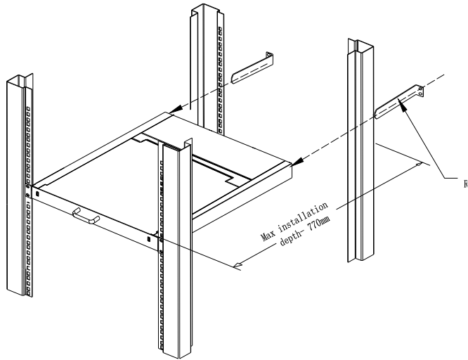
2-1.1 rack mounting (1)
