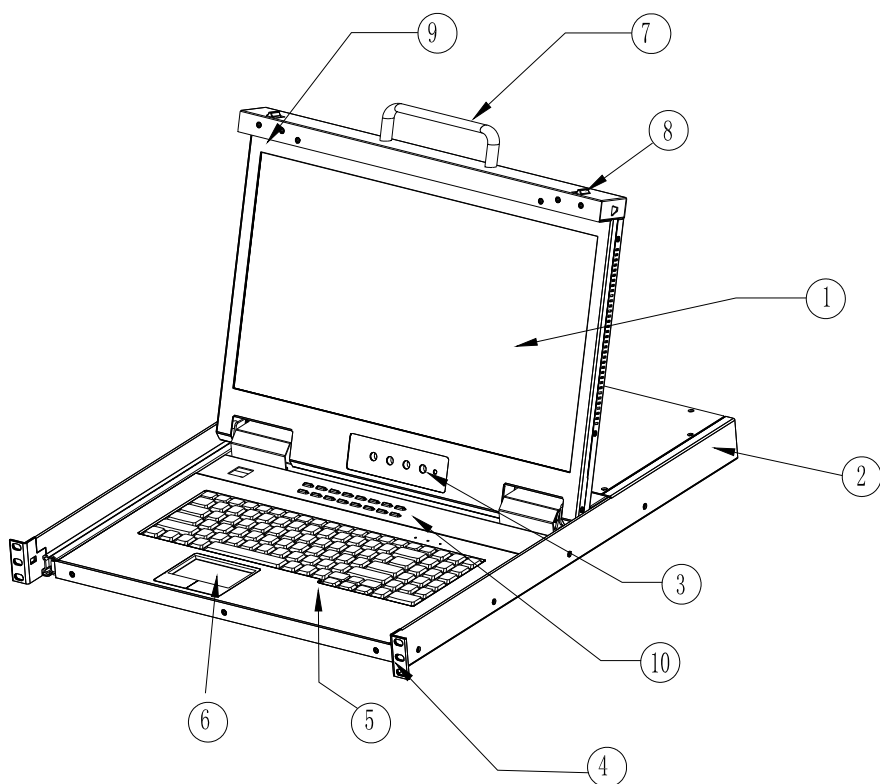
1-1.1 front view
