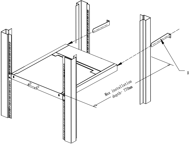
2-1.1 rack mounting (1)
