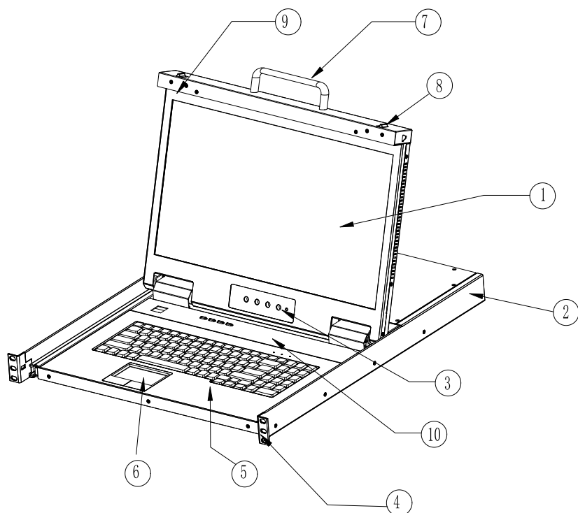
Figure 1-1.1 Front view
